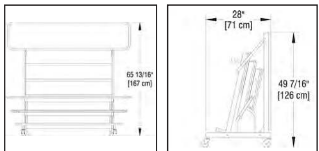
END VIEW
