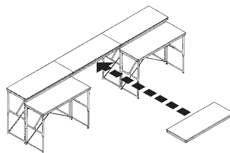
Bridge units slide into channels built into the ends of leg units.
