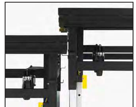
The stage sections lock together with built-in unit-to-unit connectors when units are at the same or varying heights. No cords, Velcro, straps, or tape are necessary to hold stages in place.
